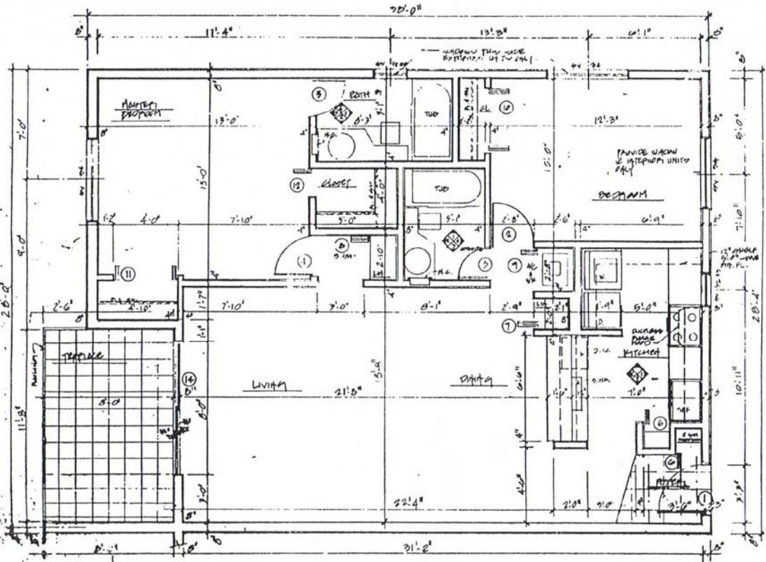
TYPICAL FLOOR PLAN CC. 9/8 = 11.0"
