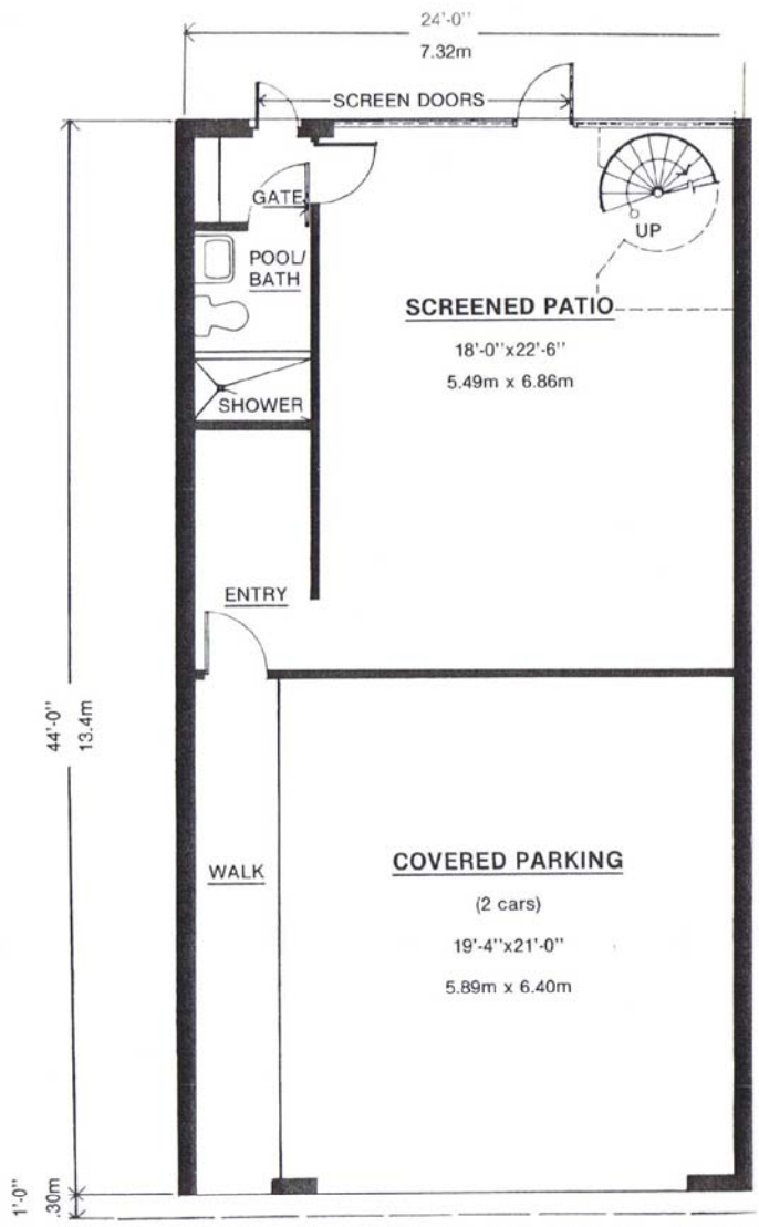
Ground Floor Plan Model F
