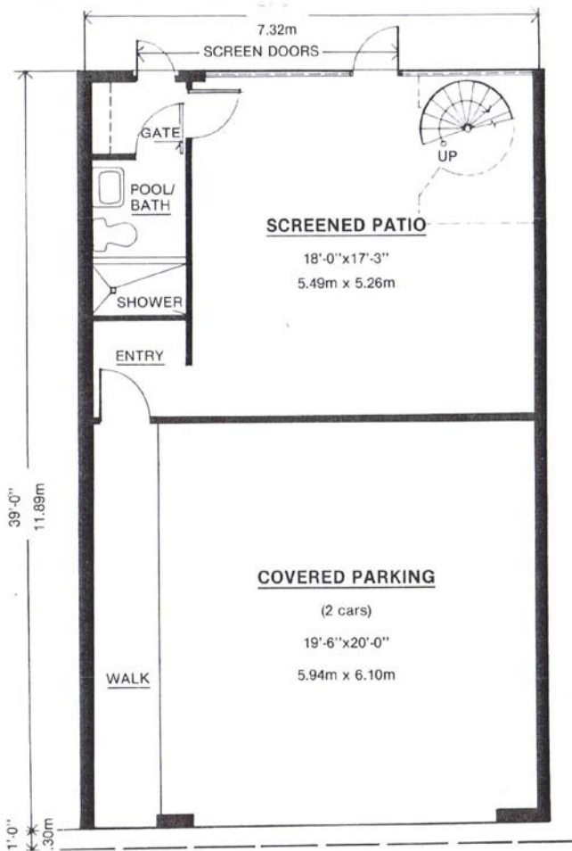
Ground Floor Plan Model E
