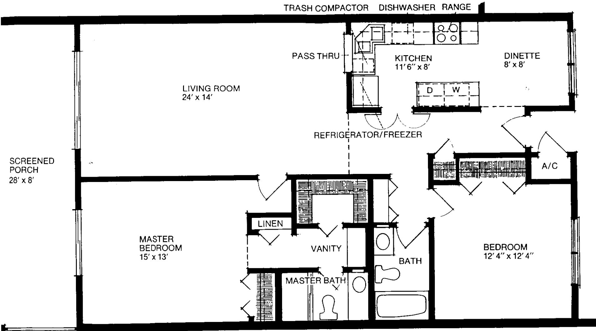
FLOOR PLAN — CENTER UNIT "B"
