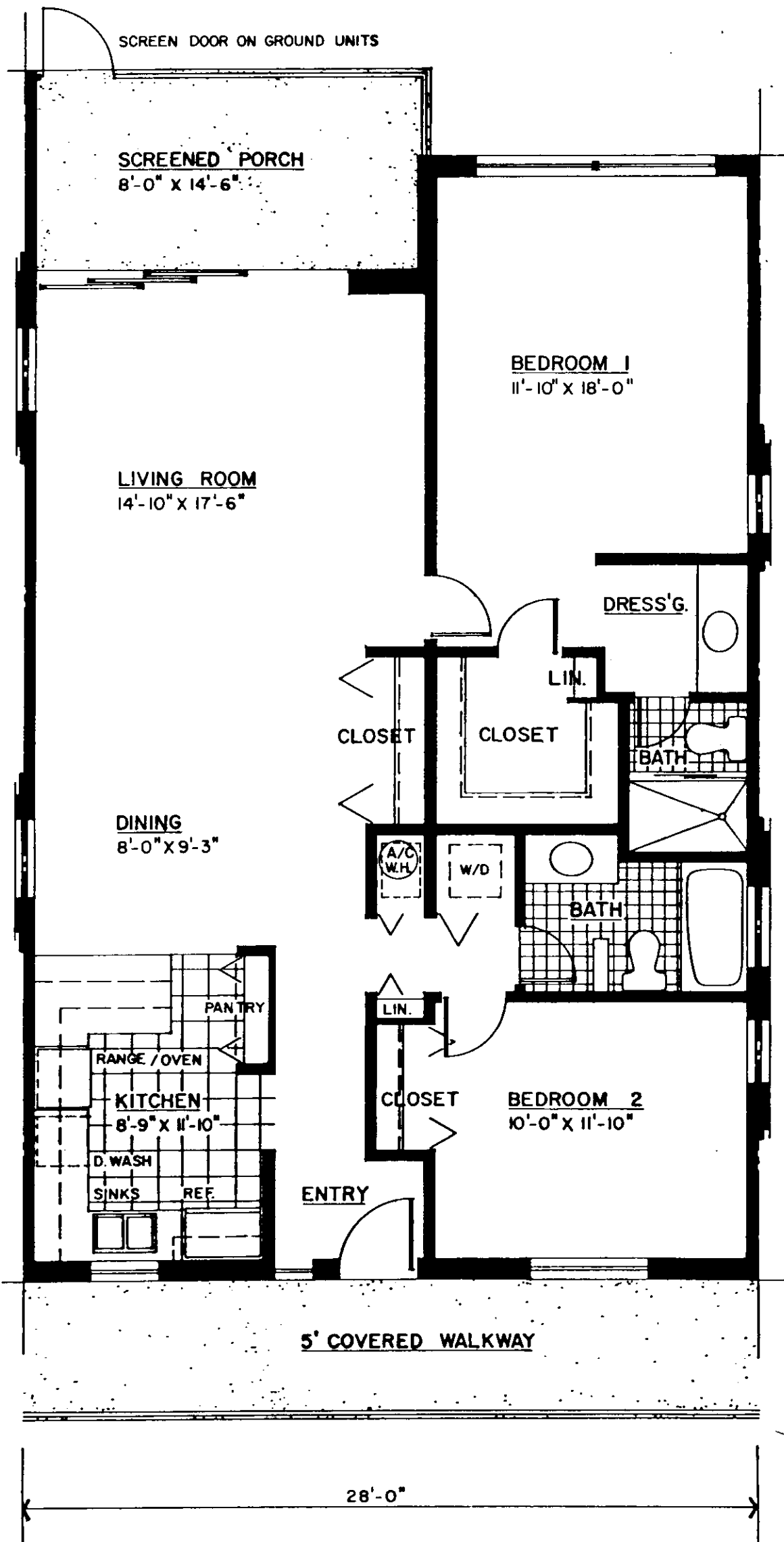
TYPICAL UNIT PLAN
