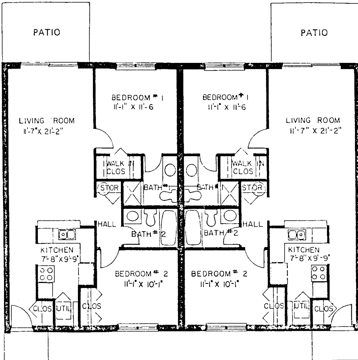
TYPICAL FIRST FLOOR UNITS BUILDING NO. 4, 5 & 6
