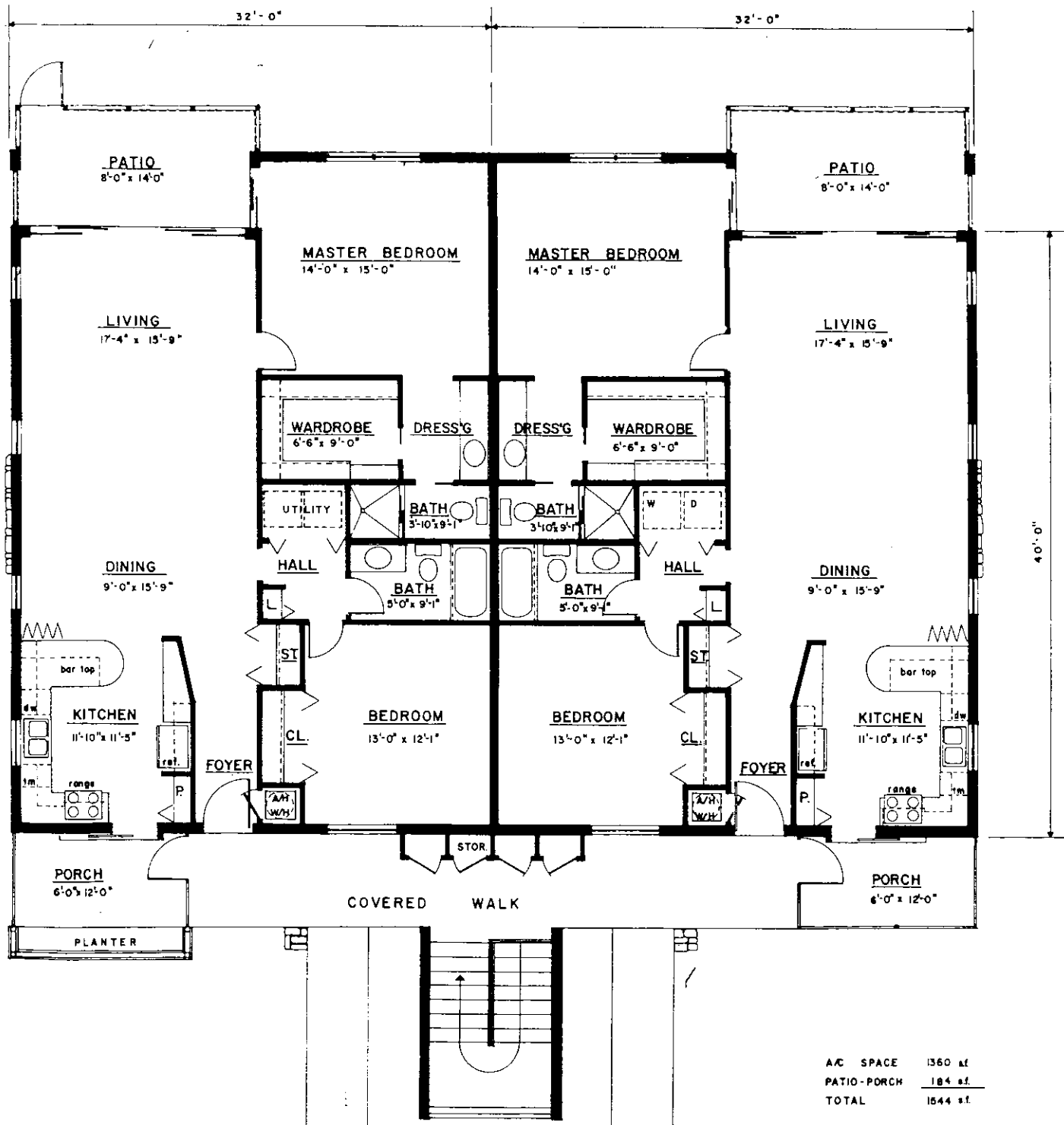
TYPICAL FLOOR PLAN BUILDING 1 AND 2
