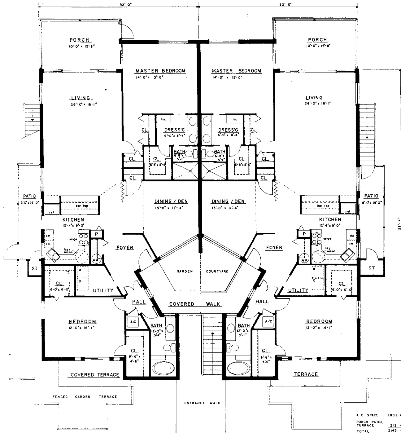
TYPICAL FLOOR PLAN BUILDING 3
