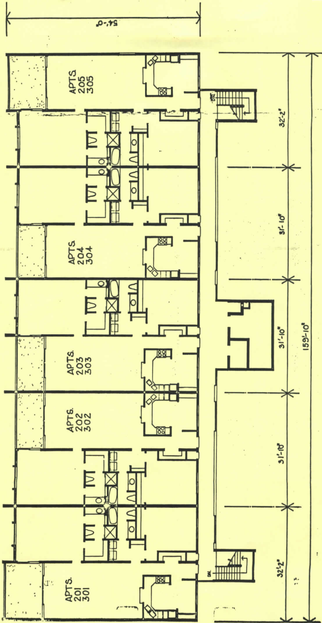
TYPICAL 2 ND & 3 RD FLOOR PLAN
